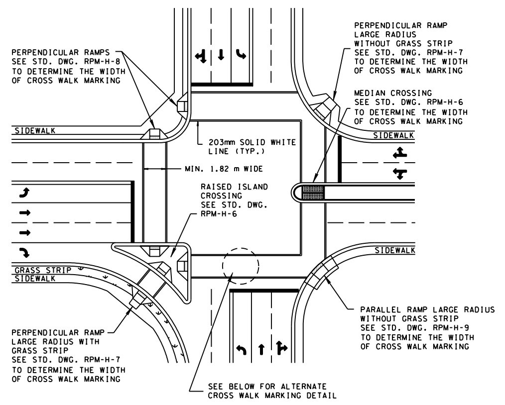
TYPICAL PLAN VIEW OF STANDARD CROSS WALK MARKING
